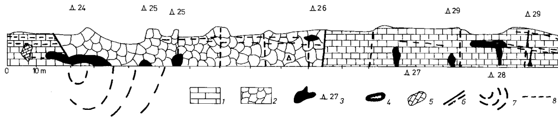
Fig. 3. Geological-geomorphological profiles in the region of the “Tyulenovo” dislocation: 1 - Sarmatian limestones; 2 - blocking; 3 - a cave with its number; 4 - a cave dwelling; 5 - olistolith; 6 - faults; 7 - event localisation; 8 - horizontal cracks and sea levels during the time of the transgression.
