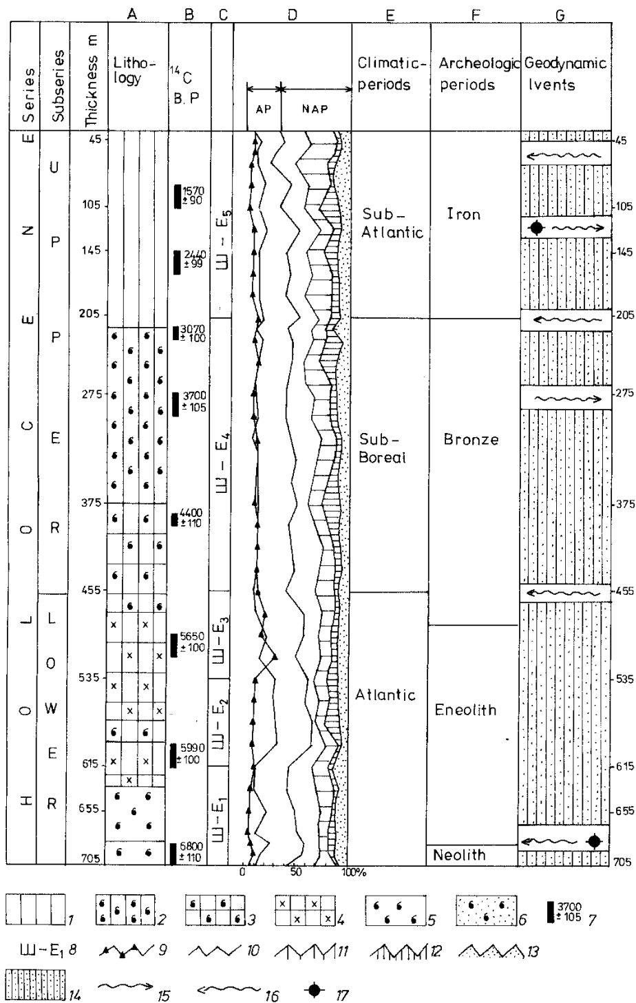
Fig. 2. Correlation scheme of the sediments and the events in the Shabla-Ezerets wetland: A. Lithological column of the lithological varieties (authors: Filipova-Marinoва, Bozhilova, 1990): 1 – peat; 2 – peat with mollusca; 3 – gyttja with mollusca; 4 – gyttja; 5 – mollusca; 6 – mollusca with sand; B. Radiocarbon datings of Prof. Delibrias, France: 7 – 14 c. B.P. (in Filipova-Marinoва, Bozhilova, 1990); C – 8 – Spore-pollen zones (authors: Filipova-Marinoва, Bozhilova, 1990); D – Spore-pollen diaframs (authors: Filipova-Marinoва, Bozhilova, 1990): 9 – Quercus ; 10 Carpinus betulus ; 11 – Poaceae ; 12 – Chenopodiaceae ; 13 – Artemisia ; E – Climatic periods (according to Blit-Sercander); F – Archeological periods (according to Todorova, 1979); G – Geodynamic events: 14 – sediment deposition; 15 – regression; 16 – transgression; 17 – paleoseismic events.
