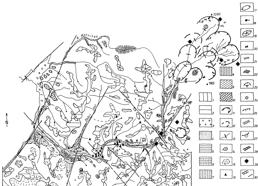
Fig. 4. Geomorphological map of the Bosnek karst region and of the upper part of the Strouma River watershed: (1-3) Plio-Pleistocene levels and terraces: 1 - I level, 2 - II level, 3 - III level; (4-10) River terraces: 4 - flood terraces, 5 -first overflow terrace, 6 - second overflow terrace, 7 - third overflow terrace, 8 - fourth overflow terrace, 9 - fifth overflow terrace, 10 - sixth overflow terrace; (11-13) Glacial forms: 11 - Basic cirque, 12 - Inserted cirque, 13 - throg step; 14 - peat marshlands; (15-17) Karst forms: 15 - karren fields, 16 - cave, 17 - vallog; 18 - springs; 19 - monadnocks,; 20 - rock dolls; 21 - rock slopes; 22 - ancient gold workings; 23 - quarry; 24 - hillock; 25 - excavation; 26 - canalised riverbed; 27 - river network rearrangement; 28 - erosion slopes; 29 - paleoseismic dislocations; 30 - normal faults and faults.
