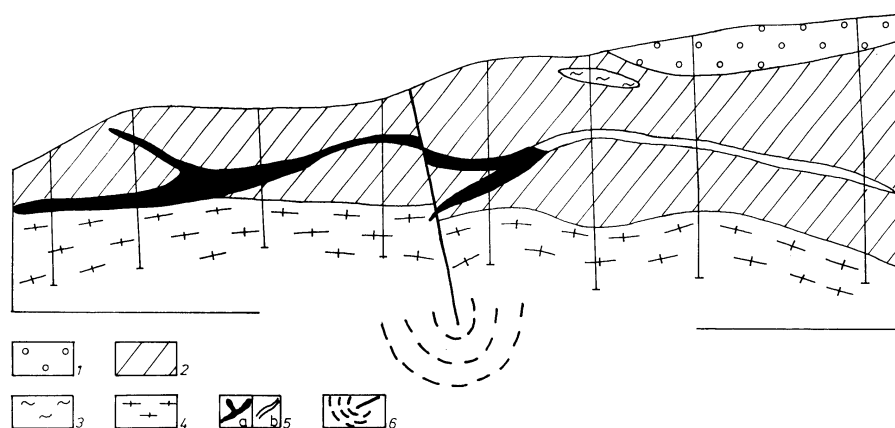
Fig. 5. Geological section across the “Yanchova River” paleoseismic dislocation: 1 – Paleogene marble breccia; 2 – marbles; 3 – biotite gneisses; 4 – granitised biotite gneisses; 5 – paleokarst (caves): a) filled, b) hollow; 6 – paleoseismic fault.
