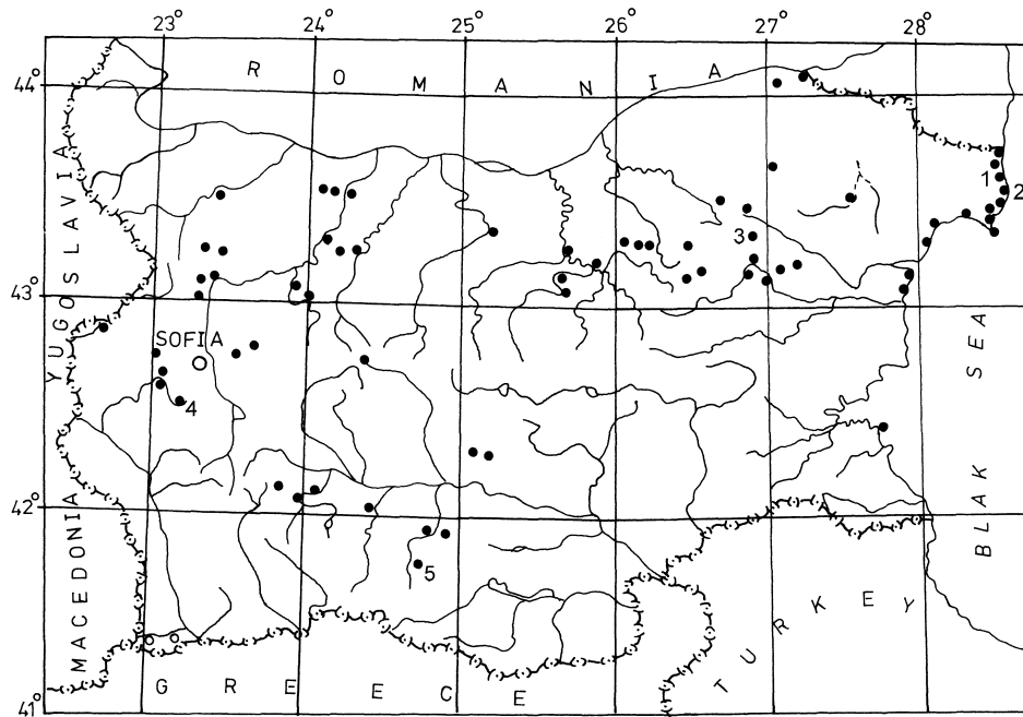
Fig. 1. Map of the paleoseismic dislocations in karst terrains in Bulgaria. (The numbers correspond to the text).
