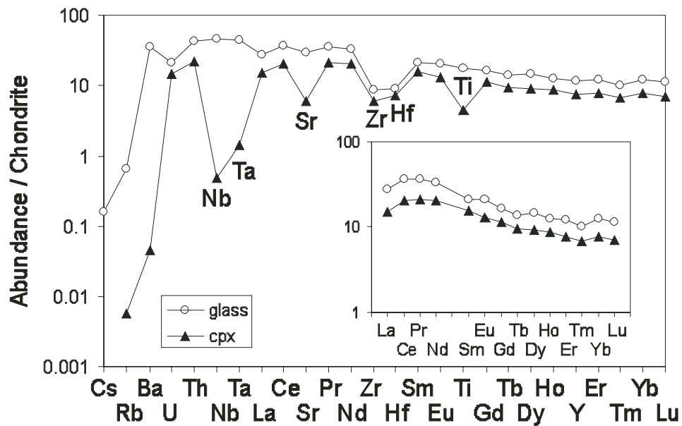
Fig. 1. Trace element composition of glass and primary clinopyroxene from Szt1130 spinel peridotite xenolith
