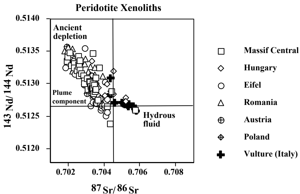
Fig.1. A compilation of isotope data for mantle peridotite xenoliths from Europe.
