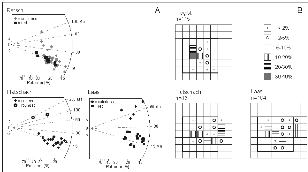
Fig. 3: A – Radial plot of zircon fission track ages from Ratsch, Flatschach and Laas.
