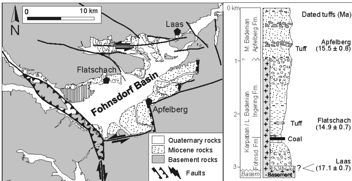
Fig. 4: Geologic map and stratigraphic section of the Fohndorf Basin with the position of tuffs.
