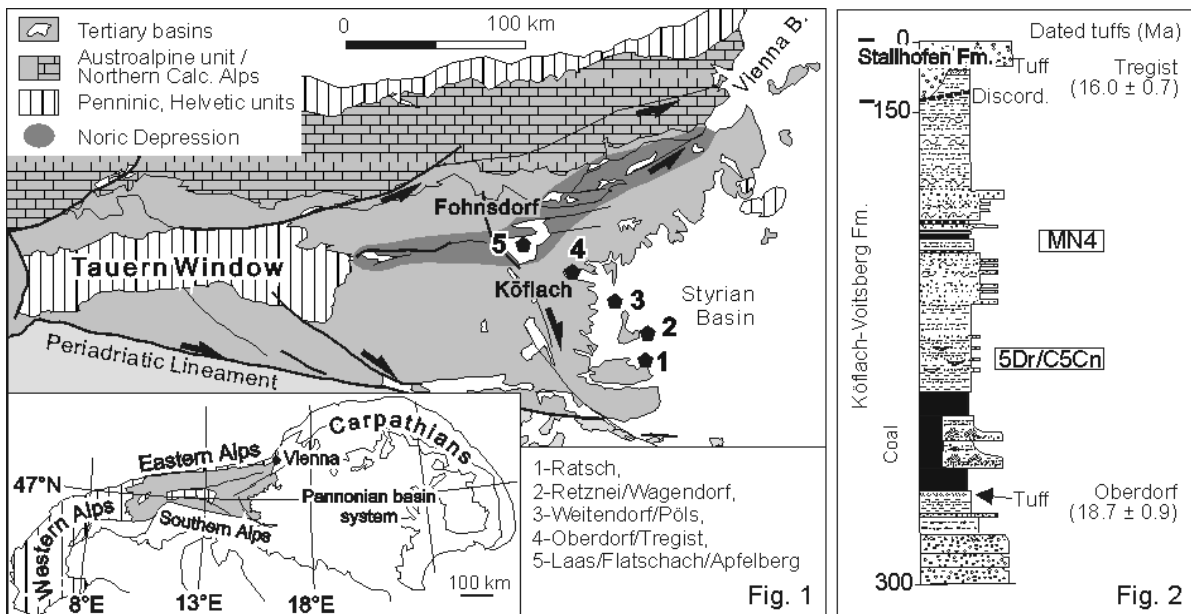
Fig. 1: Position of investigated tuffs in the Styrian Basin and the Noric Depression.
