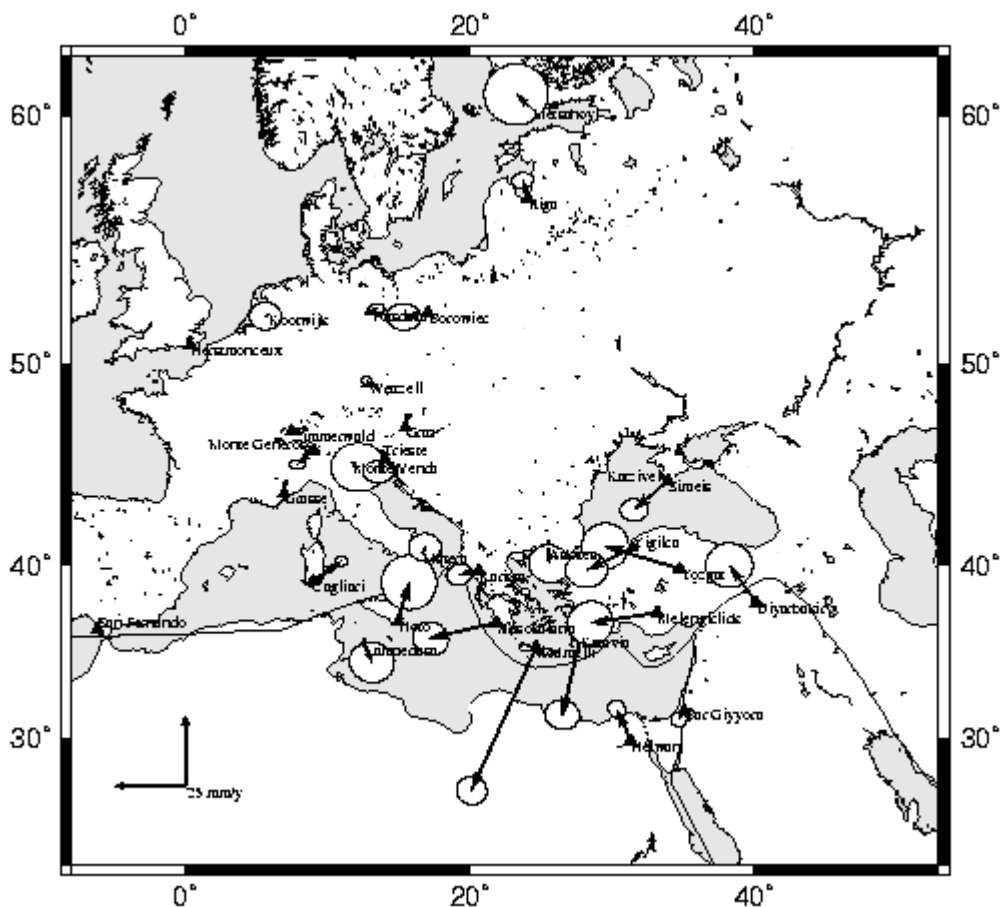
Fig. 2 Motions relative to Eurasia for the SLR stations around and in the Carpathian-Balkan Region
