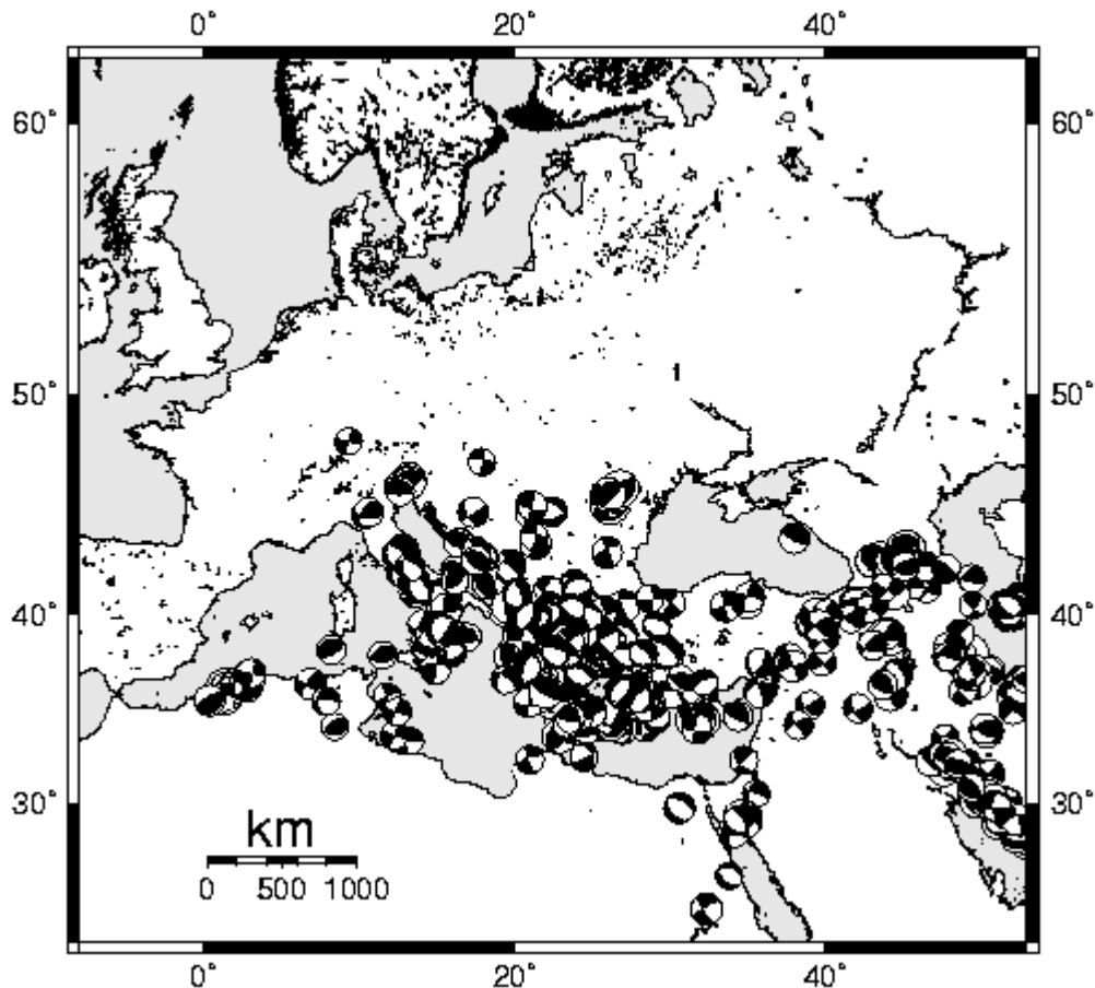
Figure 3: Fault-plane solutions from earthquakes (1977 to 2000) in the Eastern Mediterranean according to the Harvard catalogue.
