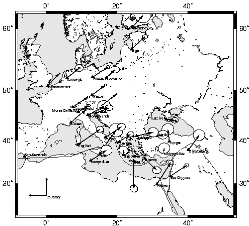
Fig. 1 Absolute motions of Europe, African and Anatolian according to SLR geodetic solution
