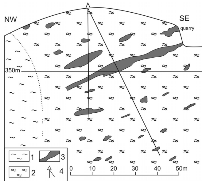
Figure 4. Geological cross-section of the Kozje Brdo deposit [4]. Legend: 1 – slightly altered serpentinite: 2 – highly altered and brecciated serpentinite: 3 – carbonate-silica breccia with agate; 4 – boreholes
