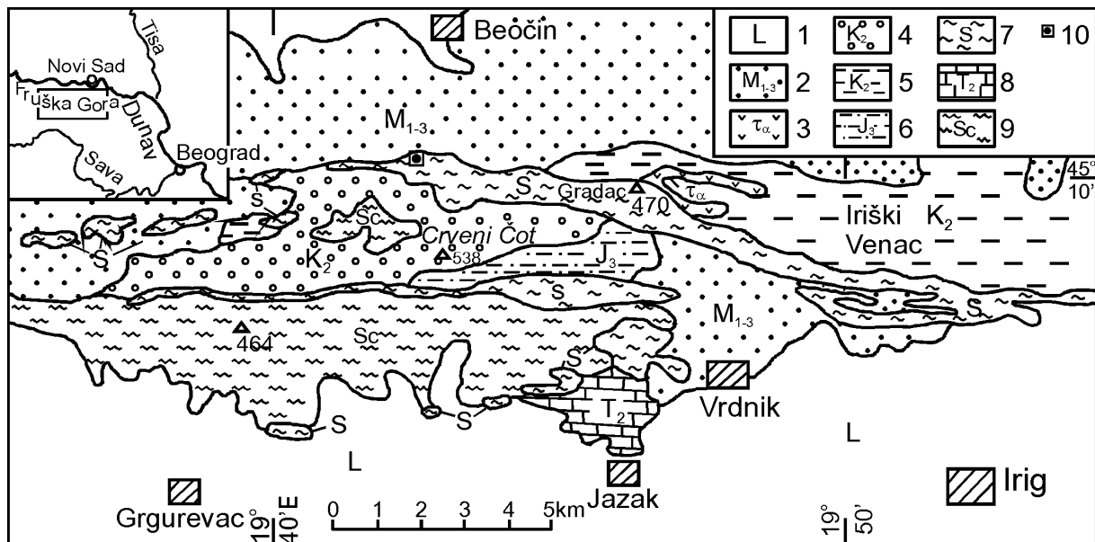
Figure 1. A sketch map of the Frushka Gora mountain (according to the Basic geological map, sheet Novi Sad). Legend: 1 – loess; 2 – Miocene marl, argillite, conglomerate and sandstone; 3 – latite; 4 – Upper Cretaceous red conglomerate and breccia; 5 – the Upper Cretaceous flysh; 6 – Jurassic slate, quartzite and sandstone; 7 – ultrabasite; 8 – Triassic argillite, limestone and dolomite; 9 – Palaeozoic sericite and chlorite schists; 10 – the Kozje Brdo deposit of gem raw materials.
