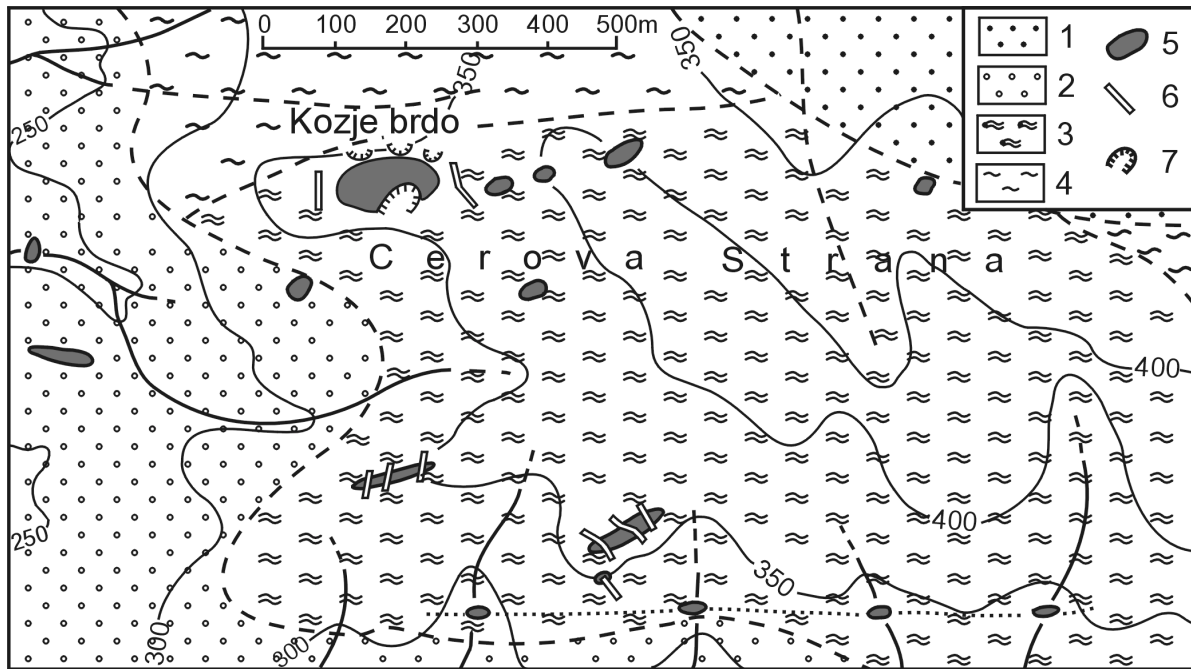
Figure 2. The ore field of Cerova Strana [4]. Legend: 1 – Tertiary gravel and clay; 2 – Upper Cretaceous red conglomerate and breccia; 3 – highly altered serpentinite; 4 – slightly altered serpentinite; 5 – Carbonate-silica breccia with agate, chalcedony; 6 – trench; 7 – quarry.
