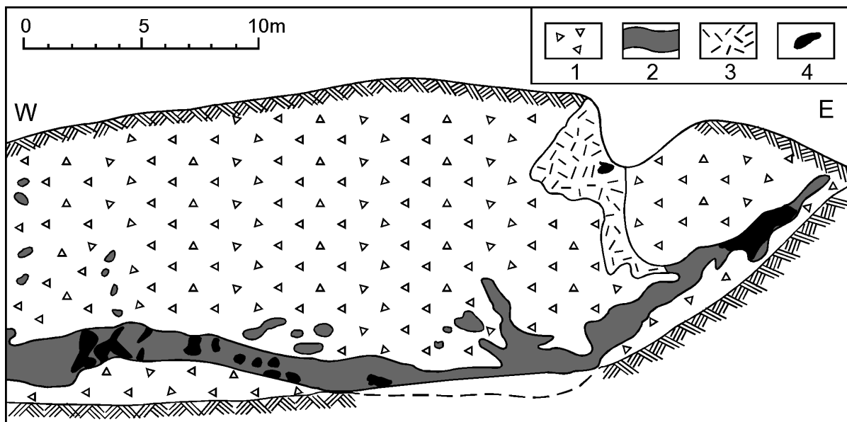
Figure 3. The open cross-section of the Kozje Brdo quarry [4]. Legend: 1 – highly altered and brecciated serpentinite; 2 – carbonate-silica breccia with agate; 3 – red-brown jasper; 4 – agate nests.
