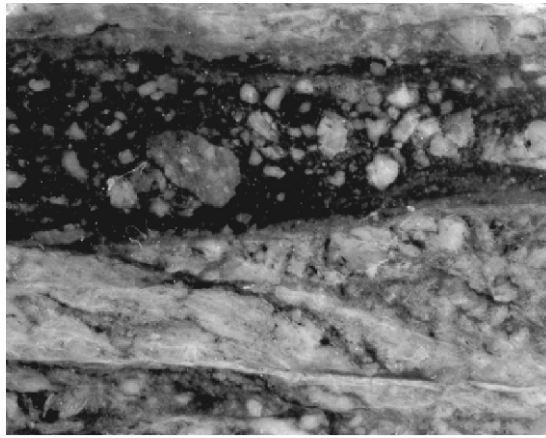
Fig. 1 Typical pseudotachylite vein sample TT-5b, width of view - 2.5 cm
