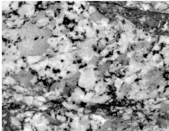
Fig. 2 Host rock biotite tonalite with small injection vein, sample TT-6a, w. - 2.5cm
