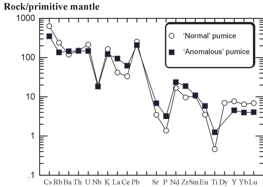
Figure 1. - Primitive mantle-normalized (data from Sun and McDonough, 1989) trace element patterns of the two types of pumices from the HIU ignimbrite
