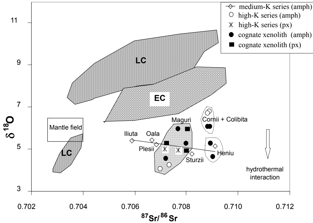
Fig. 1: \delta^{18}\text{O} (mineral separate) vs. ^{87}\text{Sr}/^{86}\text{Sr} (whole-rock) diagram for Rodna - Bârgău magmatic rocks. Bulk rock fields of Pannonian Basin lower crust (LC) (Kempton et al., 1997) and for East Carpathians (EC) including Călimani – Gurguiu – Harghita segment (Mason et al, 1996) and Ukrainian Carpathians (Seghedi et al., 2001) are also shown for comparison.
