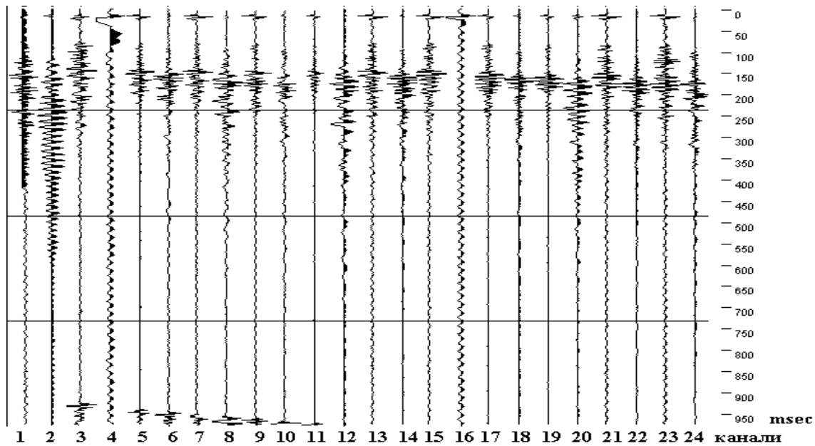
Fig. 1 Seismic records of the explosion in the hole along seismic profile No 1. The impair channels are related to vertical geophones, the pair channels are related to horizontal geophones. The first and the second geophones are inside the cave of “Dushnika”.
