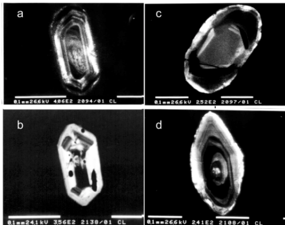
Fig. 2. CL- images of zircon from: a, c) microgranular enclaves; b) equigranular metagranites- recrystallized magmatic crystal; d) porphyritic metagranites
