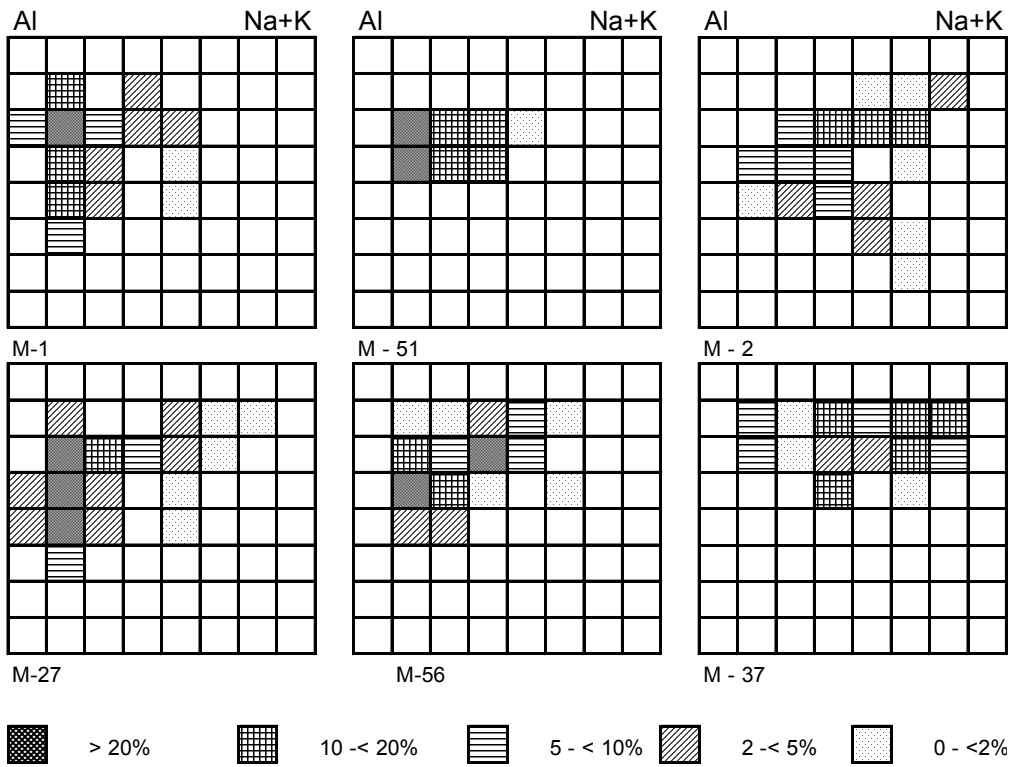
Fig. 1. Typologic distribution of the zircon populations: equigranular metagranites (M-1, M-27); porphyritic metagranites (M-51, M-56); microgranular enclaves (M-2, M-37).
