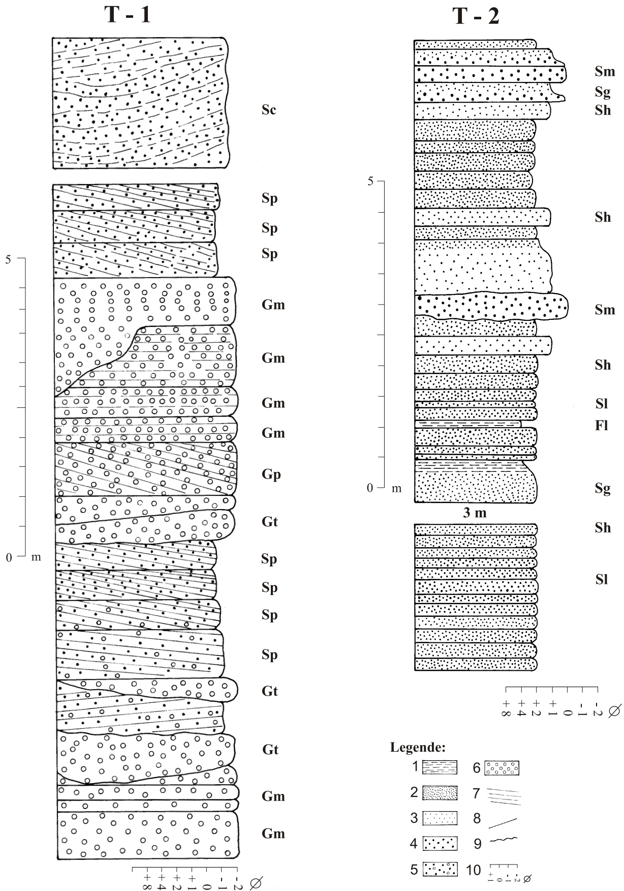
Fig. 1. Characteristic lithofacies in basal part of the Lower Triassic sequence (Locality Kostolný potok valley, SE from the Nemecká Village, Profiles T 1, T 2). Facies codes after Miall (1978).
