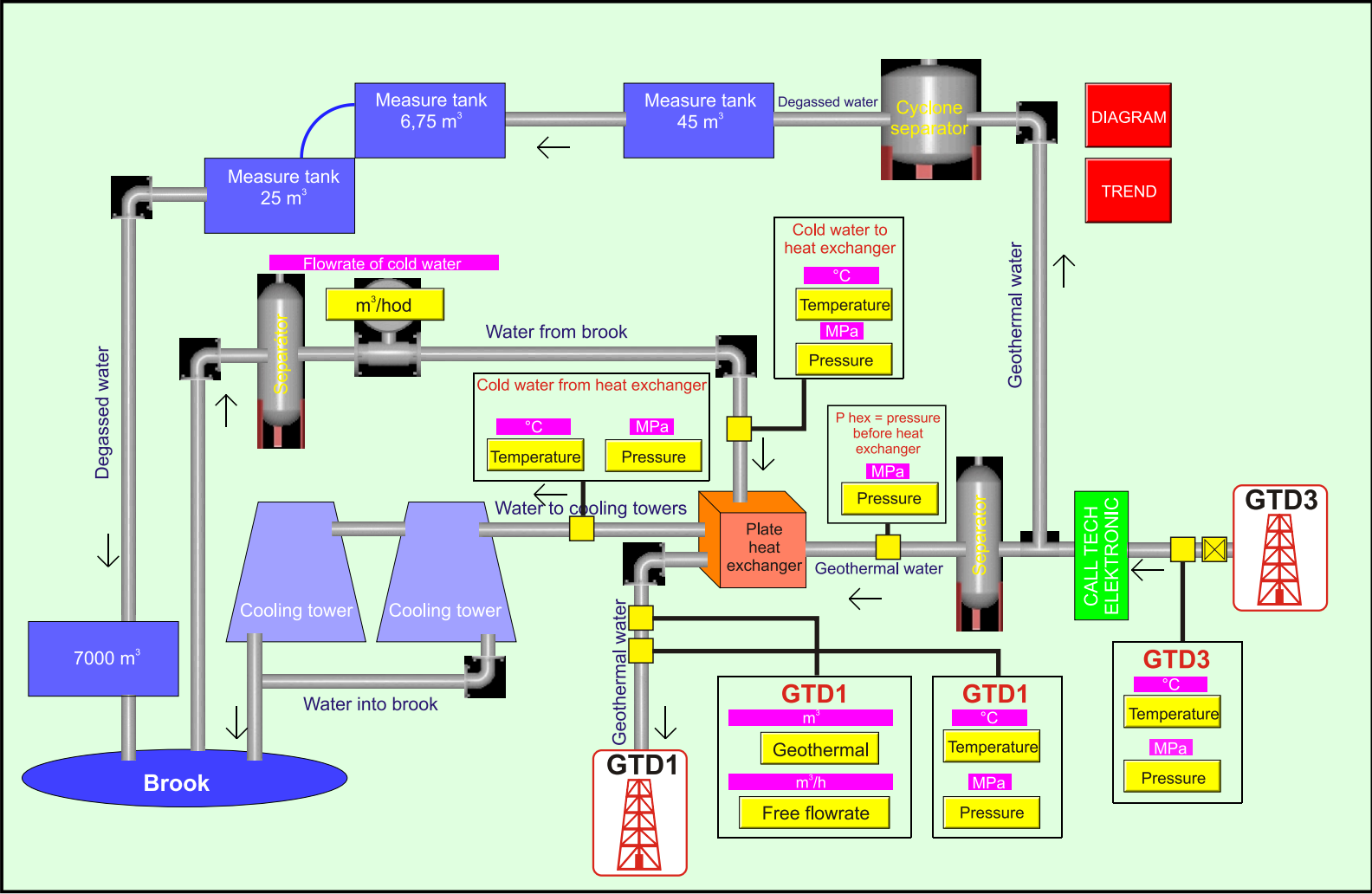
Figure 1: Scheme of the surface technology for the well test of GTD-3
