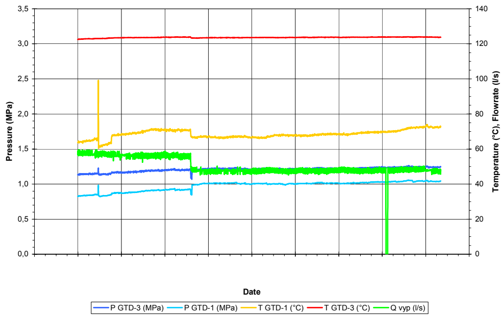
Figure 3: Hydrodynamic test on GTD-3 - geothermal loop (17 th - 27 th March 2001)
