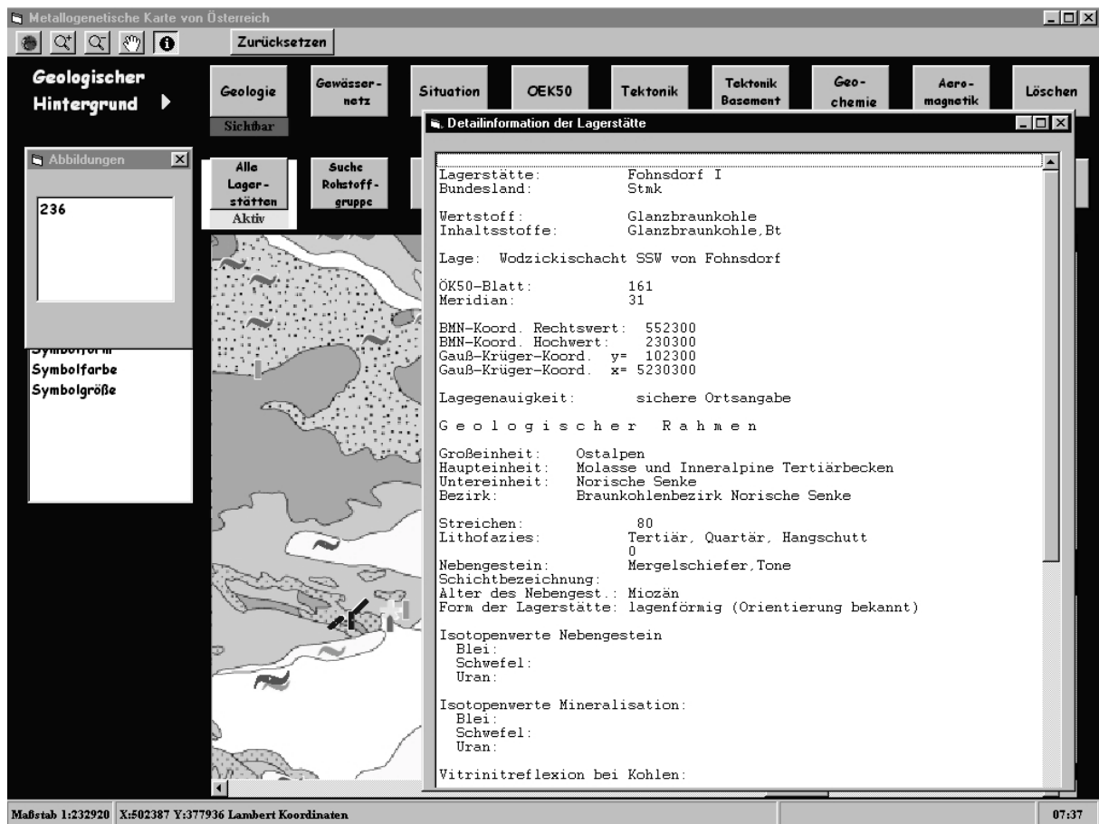
Fig. 3: Detailed information concerning “Fohnsdorf lignite deposit”.
