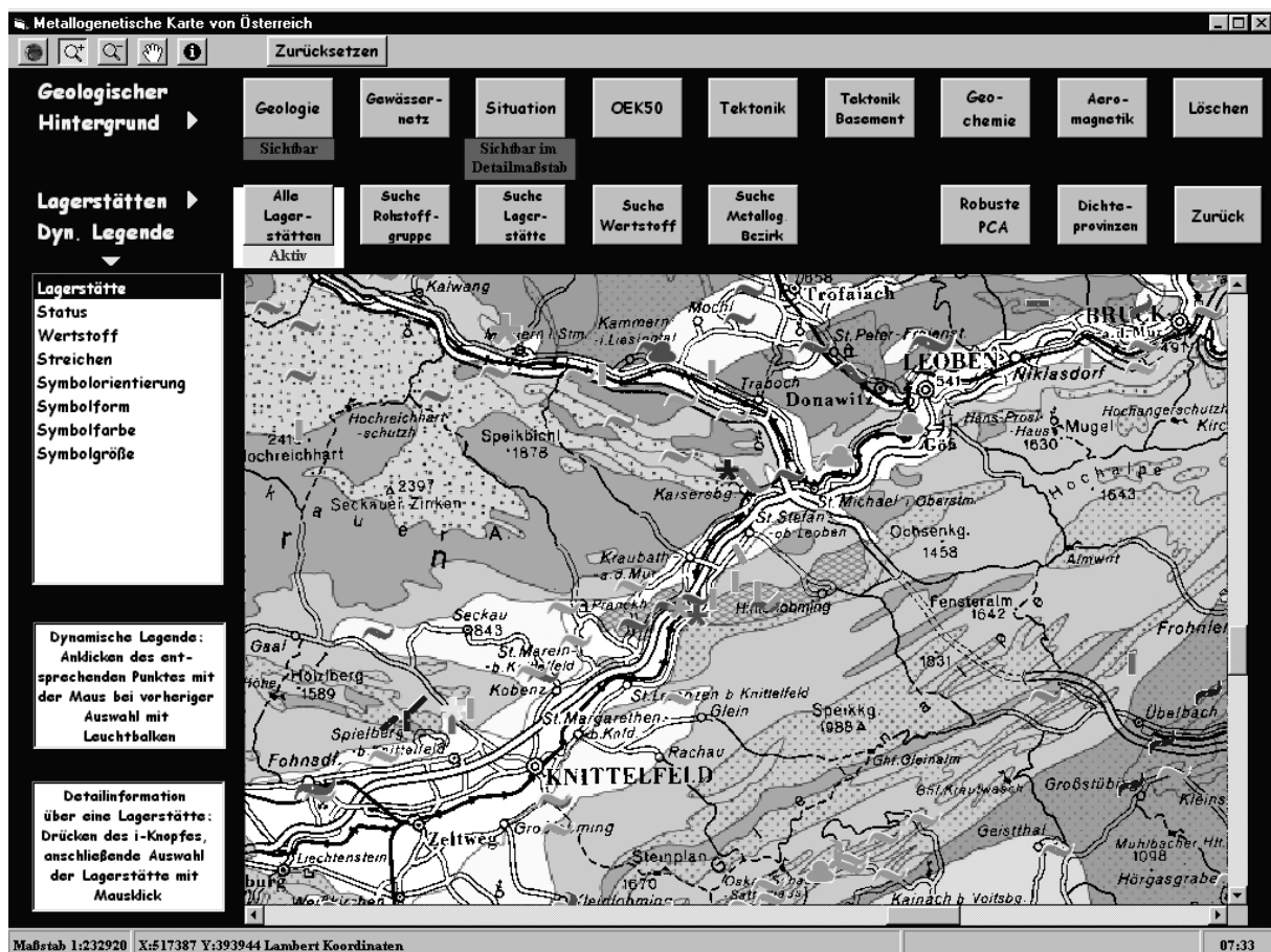
Fig. 1: Layers: Geology, mineralizations, situation (Mur Valley, Fohnsdorf/Knittelfeld Miocene Basin within the Middle Austroalpine crystalline complex).
