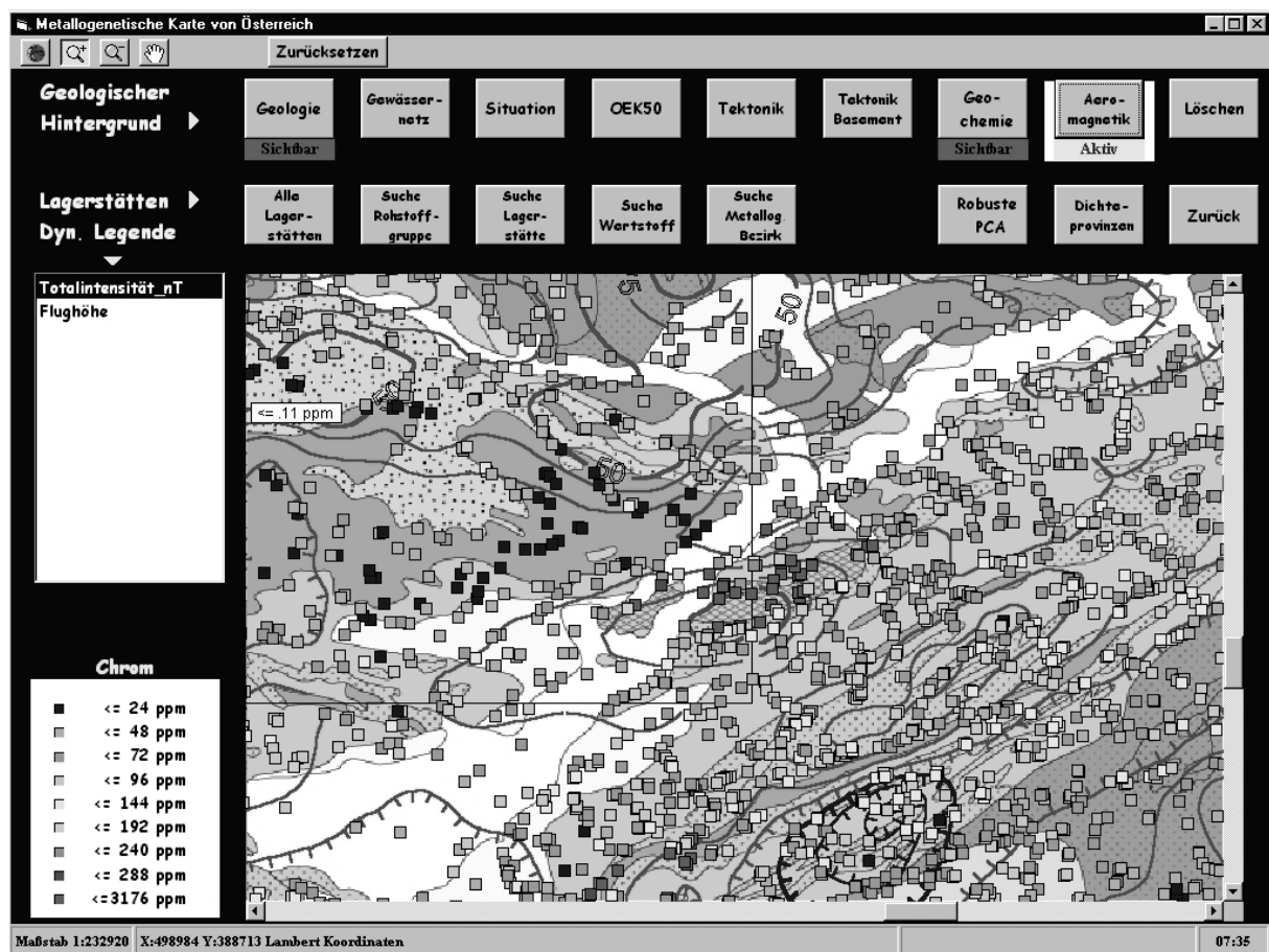
Fig. 2: Layers: Geology, geochemistry (Chromium), aeromagnetics (same area as in Fig.1).
